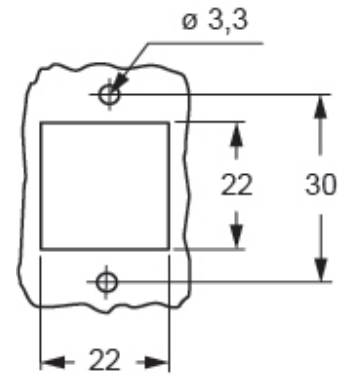
Catalogue drawings
