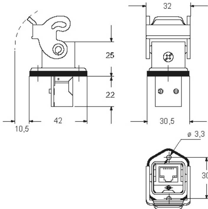
Catalogue drawings
