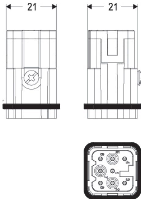
Catalogue drawings
