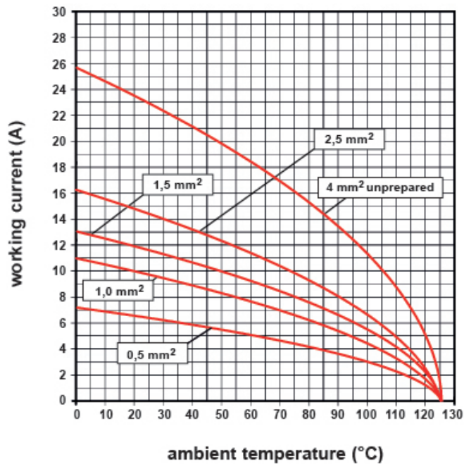
CQEY 64 poles connector inserts Maximum current load derating diagram
