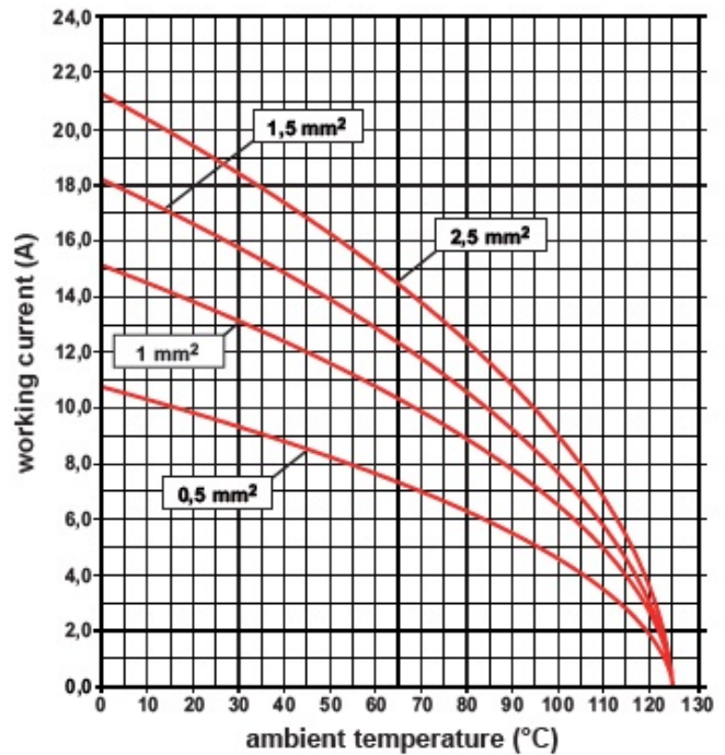
Derating curves
