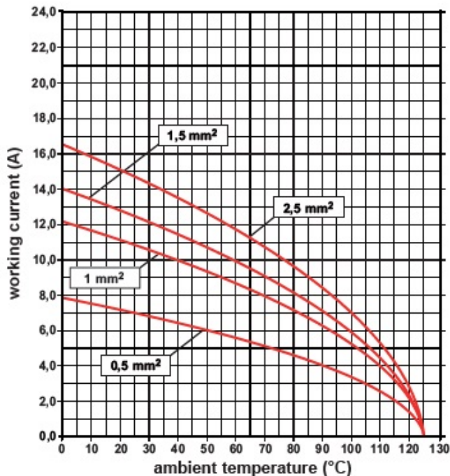
Derating curves
