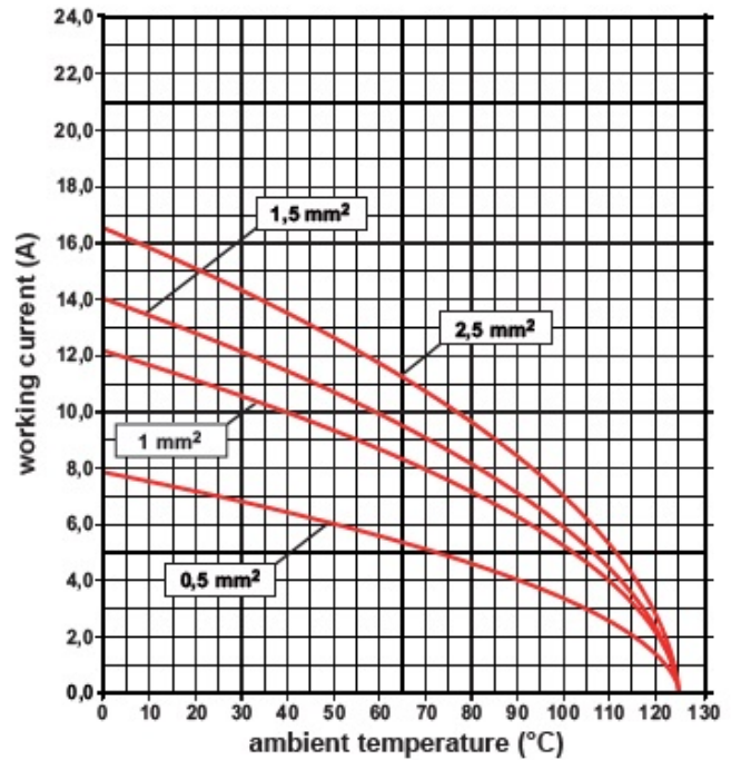
Derating curves
