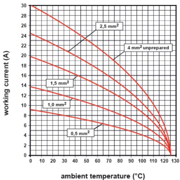
CQEYM 10 poles connector inserts Maximum current load derating diagram
