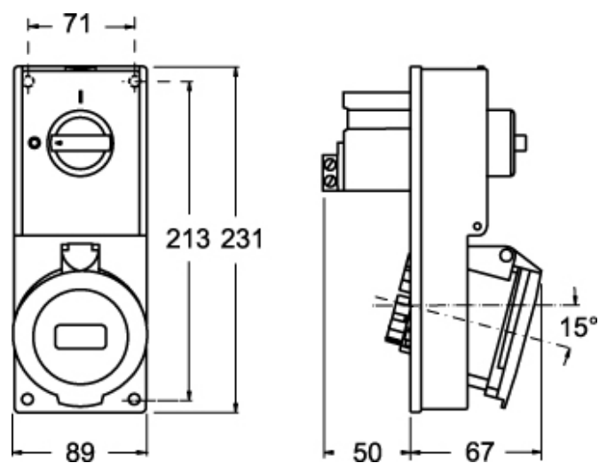
Catalogue drawings
