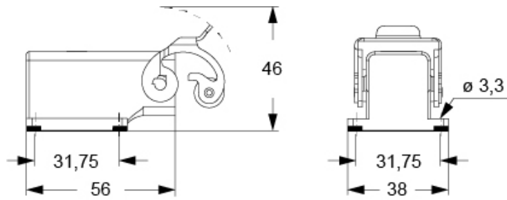
Catalogue drawings
