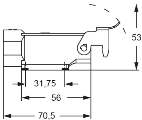
Catalogue drawings
