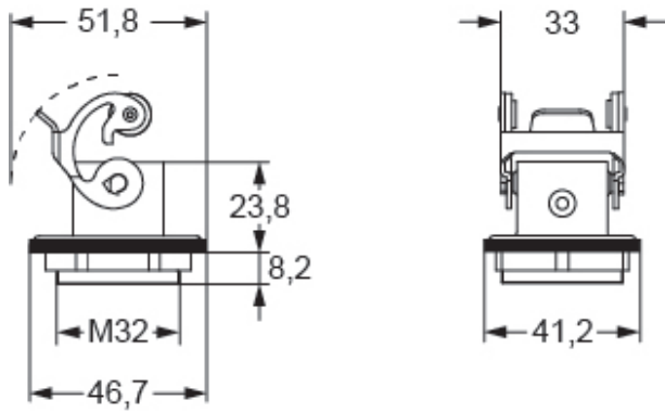
Catalogue drawings
