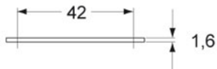
Catalogue drawings
