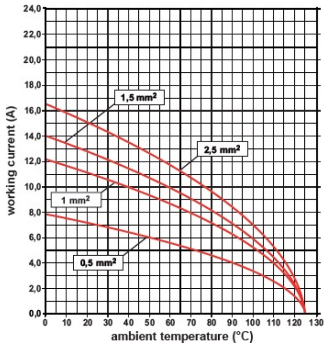
Derating curves
