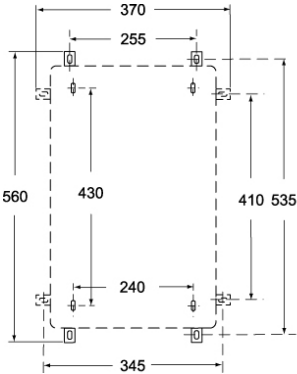
Catalogue drawings
