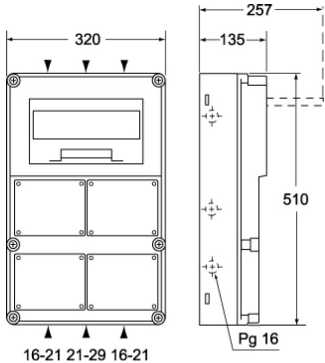
Catalogue drawings
