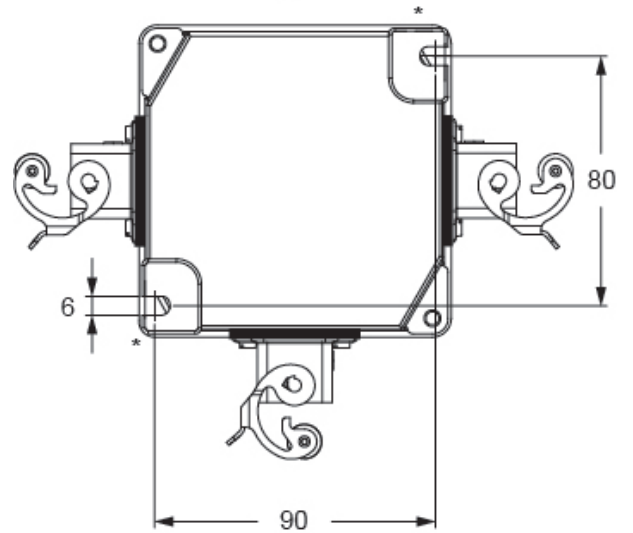
* Fixing holes
