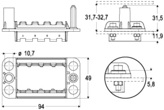
Catalogue drawings
