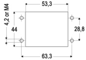
Catalogue drawings
