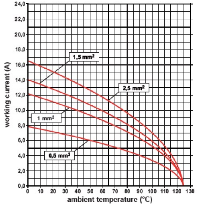
Derating curves
