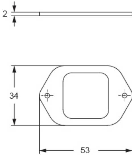
Catalogue drawings
