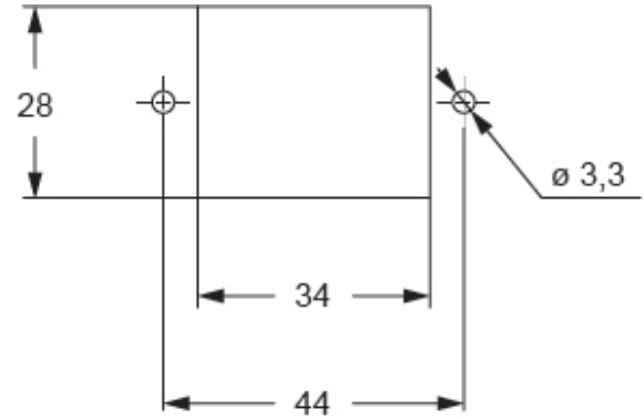
Catalogue drawings
