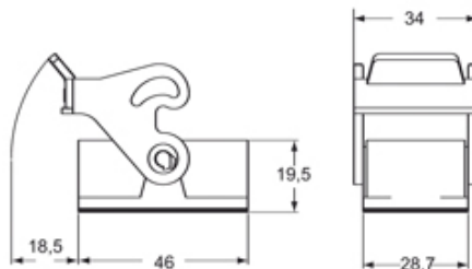
Catalogue drawings
