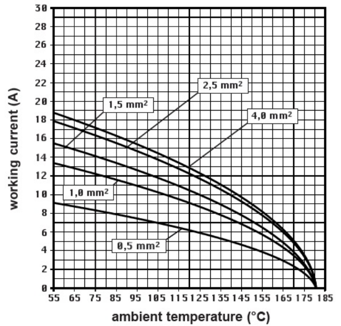
Derating curves
