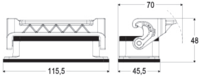
Catalogue drawings
