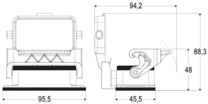
Catalogue drawings
