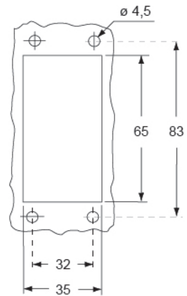
Catalogue drawings
