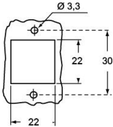
Catalogue drawings
