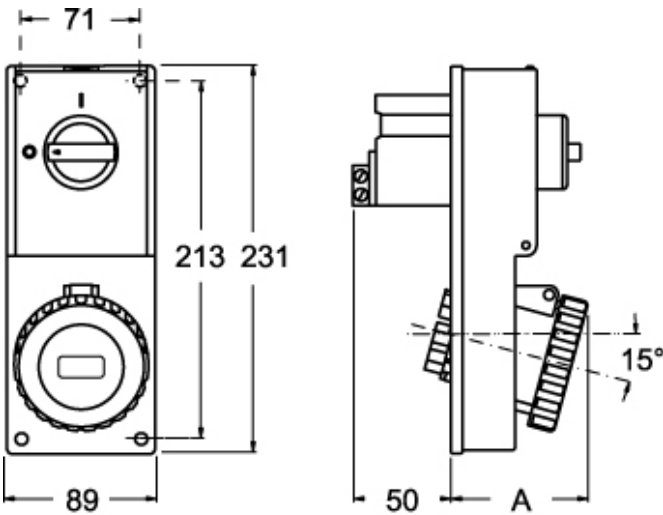
Catalogue drawings
