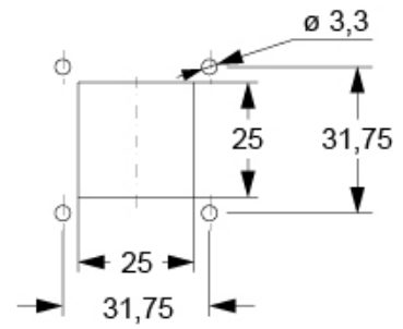
Catalogue drawings
