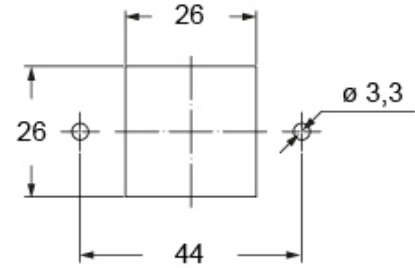
Catalogue drawings
