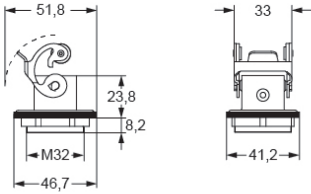
Catalogue drawings
