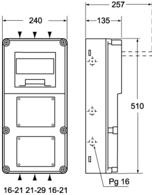
Catalogue drawings
