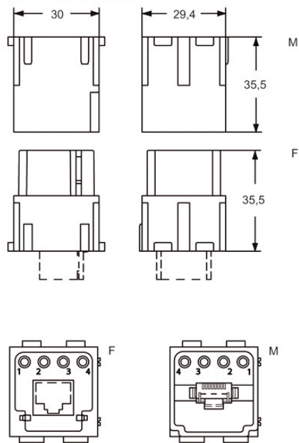
CX 01 JF, CX 01 JM
