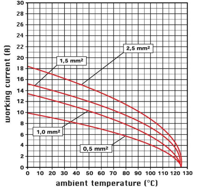
diagram CSH 24 poles
