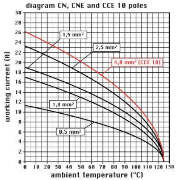
Catalogue drawings
