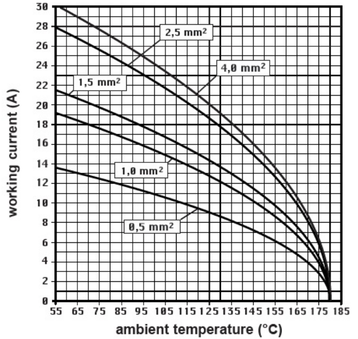
Derating curves
