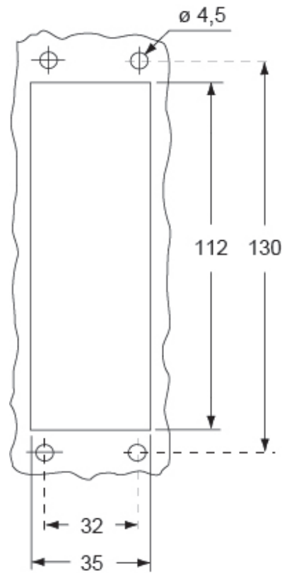
Catalogue drawings
