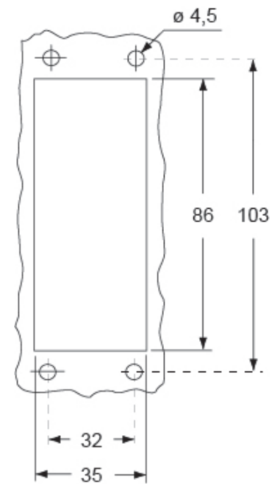
Catalogue drawings
