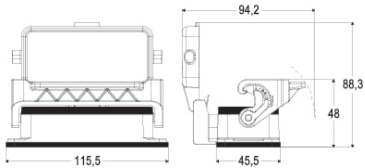
Catalogue drawings
