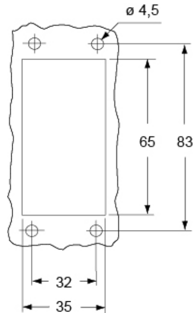
Catalogue drawings
