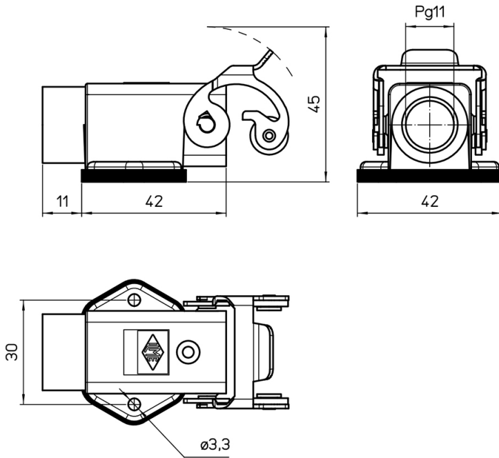
Catalogue drawings
