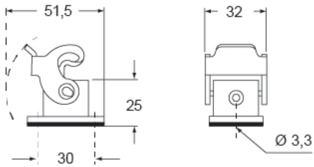
Catalogue drawings
