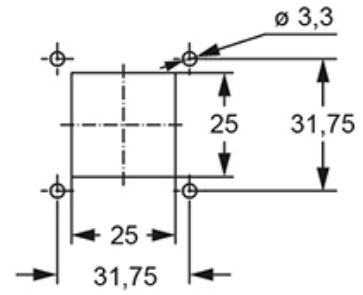
Catalogue drawings
