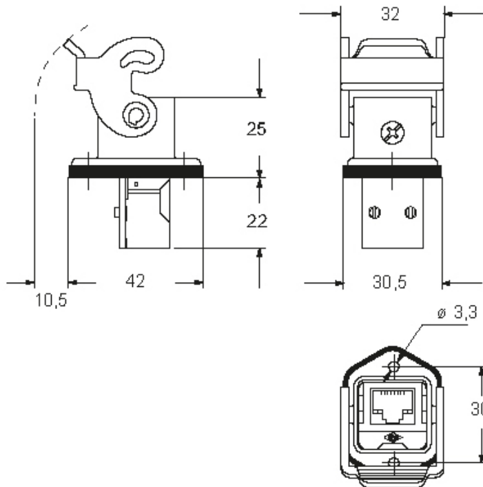
Catalogue drawings
