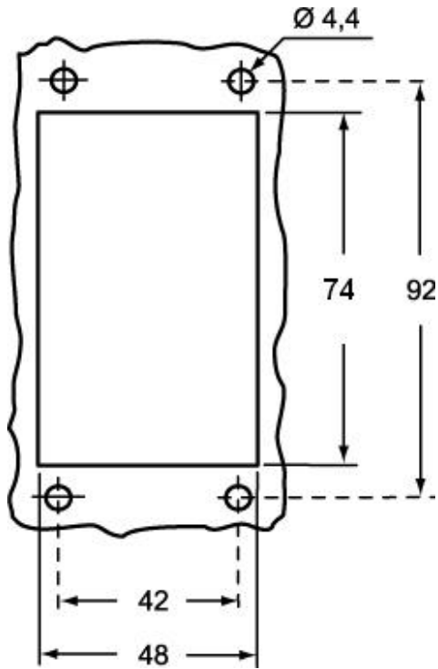
Catalogue drawings
