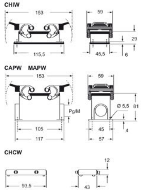
Catalogue drawings
