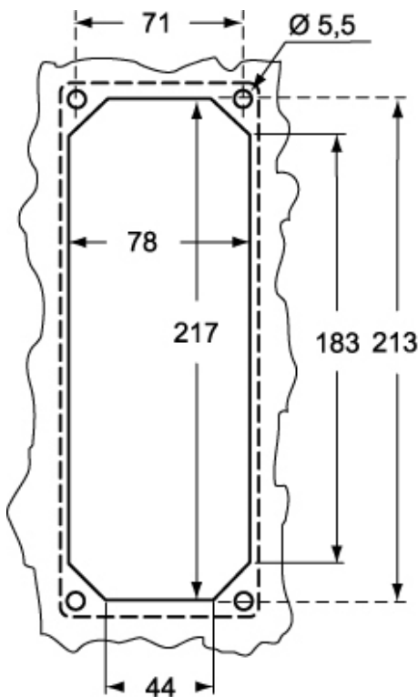
Catalogue drawings
