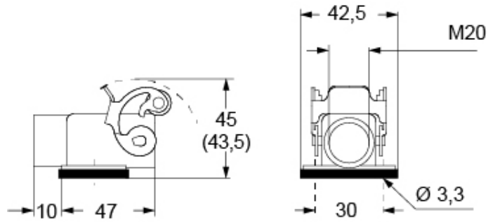
Catalogue drawings
