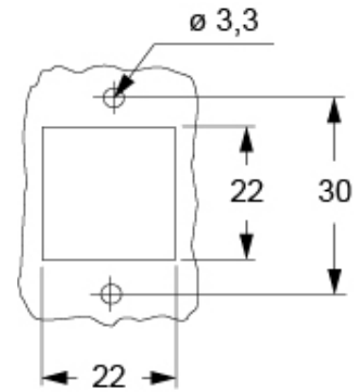
Catalogue drawings
