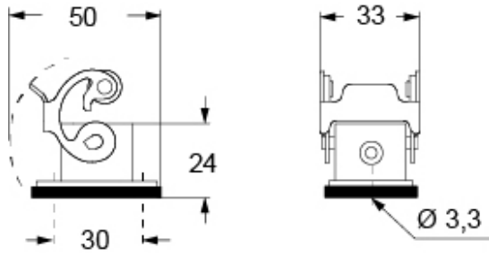
Catalogue drawings
