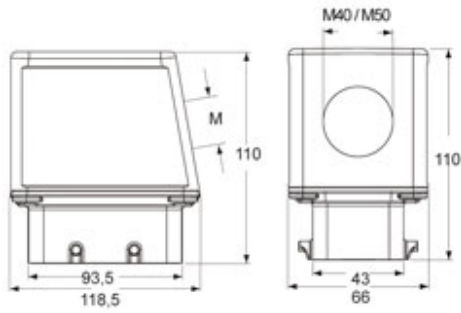
Catalogue drawings
