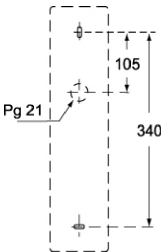
Catalogue drawings
