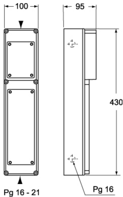
Catalogue drawings
