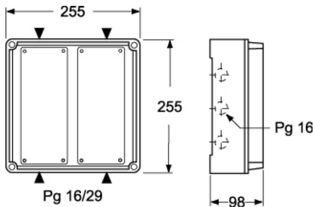
Catalogue drawings
