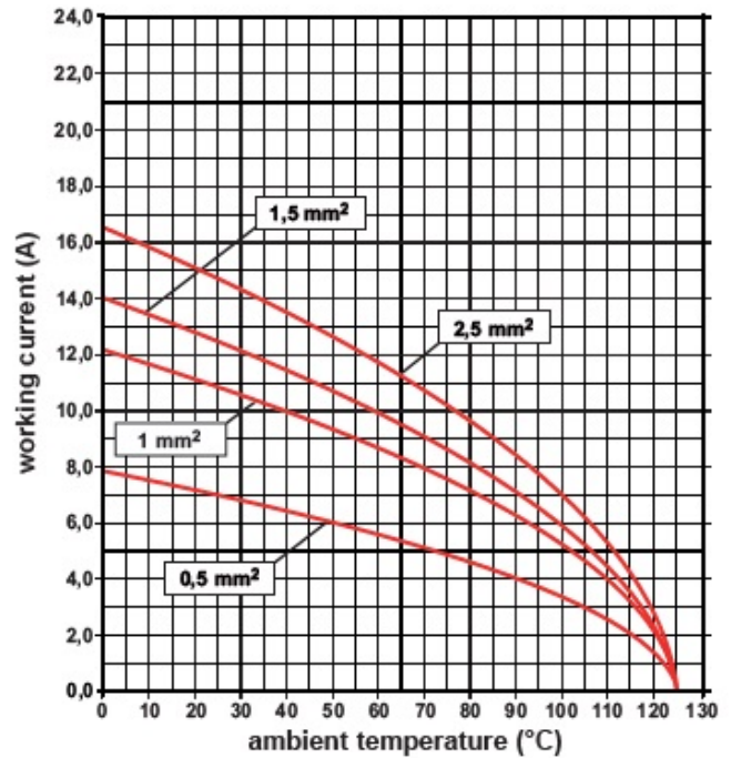
Derating curves
